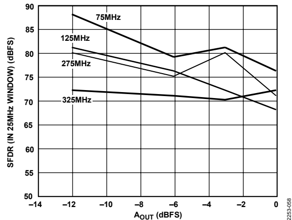
Figure 58. Dual-Tone Windowed SFDR vs. A_{OUT} at f_{DATA} = 100 MSPS
