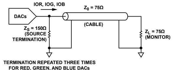
Figure 7. Analog Output Termination for RS-170
