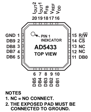
Figure 6. AD5433 Pin Configuration (LFCSP)
