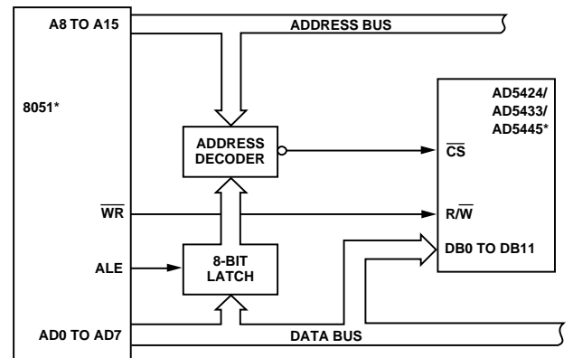
Figure 57. 8xC51-to-AD5424/AD5433/AD5445 Interface
