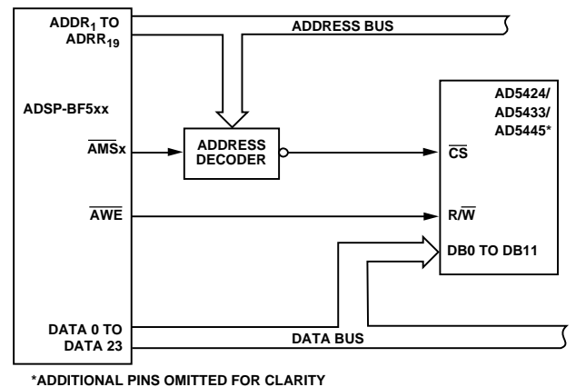
Figure 58. ADSP-BF5xx-to-AD5424/AD5433/AD5445 Interface
