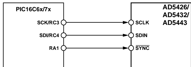
Figure 58. PIC16C6x/7x-to-AD5426/AD5432/AD5443 Interface
