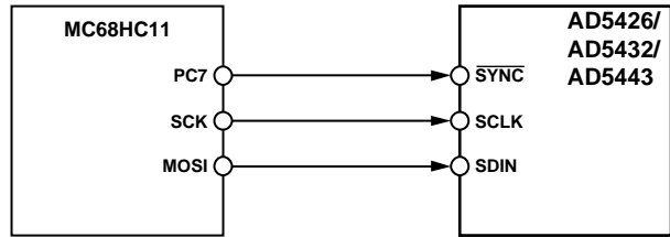
Figure 56. 68HC11/68L11-to-AD5426/AD5432/AD5443 Interface MICROWIRE to AD5426/AD5432/AD5443 Interface
