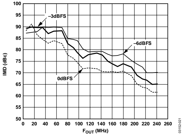
Figure 21. Third-Order IMD vs. Frequency, f_{DATA} = 62.5 \text{ MSPS} , 8\times Interpolation
