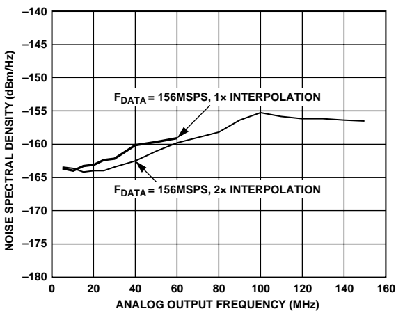
Figure 23. Noise Spectral Density vs. Analog Input Frequency, f_{DATA} = 156 \text{ MSPS}
