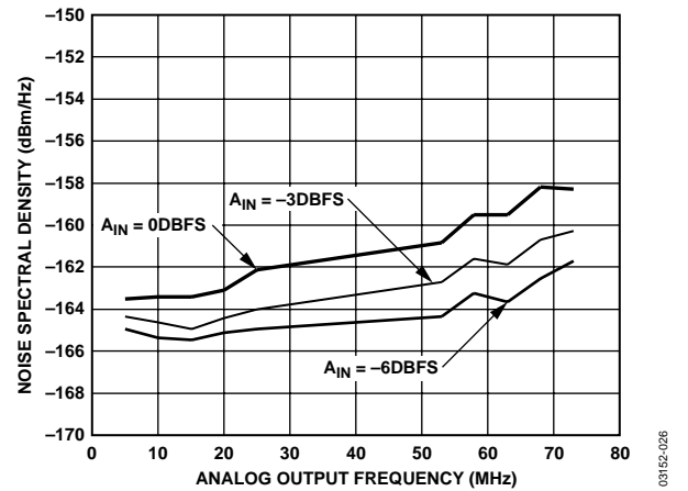
Figure 26. Noise Spectral Density vs. Analog Input Frequency, f_{DATA} = 78 \text{ MSPS} , 2\times Interpolation
