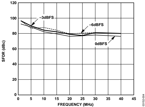
Figure 4. SFDR vs. Frequency, f_{DATA} = 100 MSPS, 4× Interpolation
