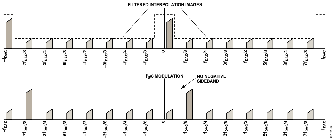
Figure 63. Complex Modulation
