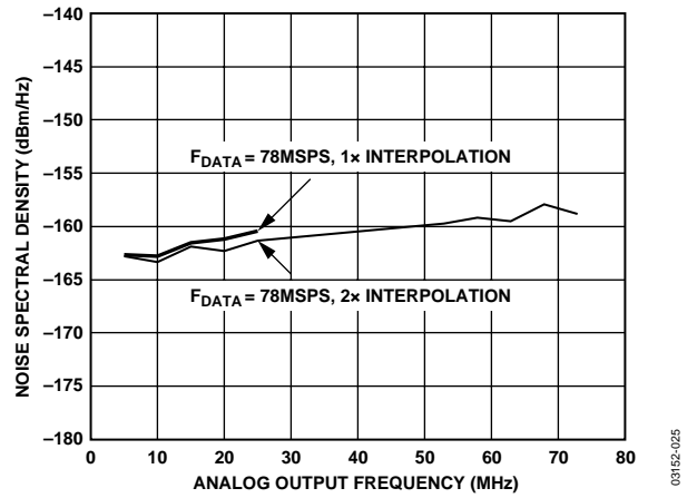
Figure 25. Noise Spectral Density vs. Analog Input Frequency, f_{DATA} = 78 \text{ MSPS}
