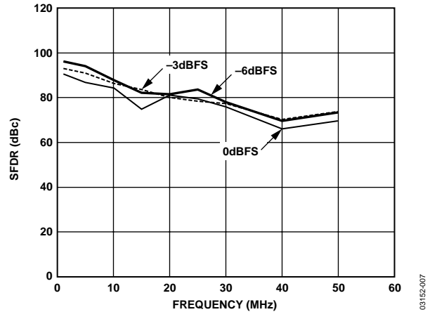
Figure 7. SFDR vs. Frequency, f_{DATA} = 125 MSPS, 4× Interpolation
