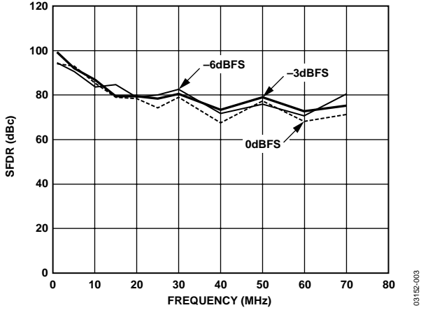
Figure 3. SFDR vs. Frequency, f_{DATA} = 200 MSPS, 1× Interpolation
