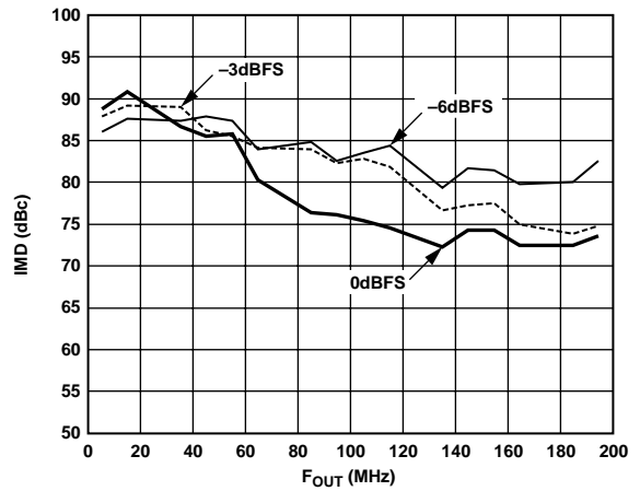
Figure 20. Third-Order IMD vs. Frequency, f_{DATA} = 50 MSPS, 8x Interpolation
