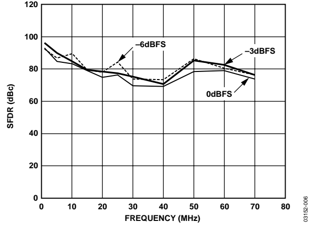
Figure 6. SFDR vs. Frequency, f_{DATA} = 200 MSPS, 2× Interpolation
