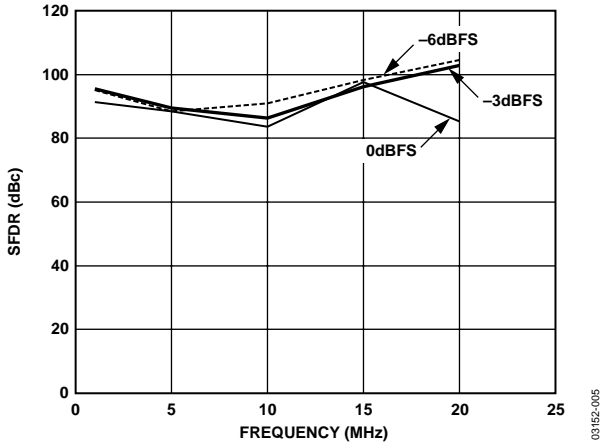
Figure 5. SFDR vs. Frequency, f_{DATA} = 50 MSPS, 8× Interpolation
