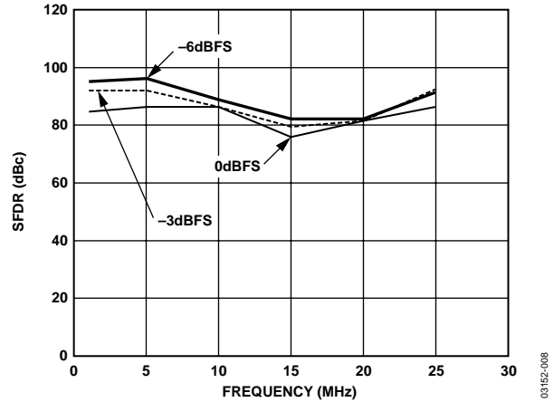
Figure 8. SFDR vs. Frequency, f_{DATA} = 62.5 MSPS, 8× Interpolation
