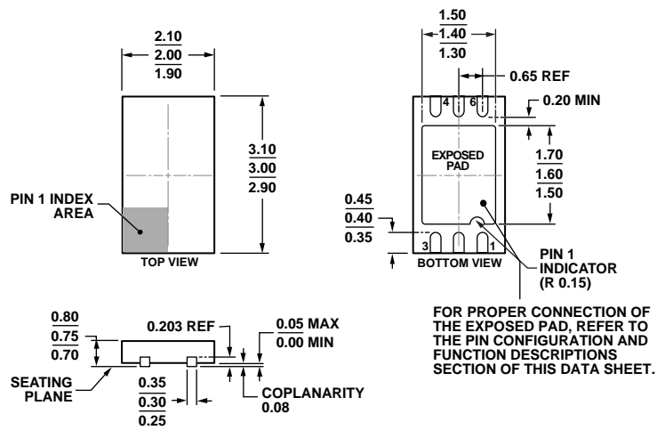
Figure 55. 6-Lead Lead Frame Chip Scale Package [LF CSP] (CP-6-5) 2.00 × 3.00 mm Body, Very Very Thin, Dual Lead Dimensions shown in millimeters
