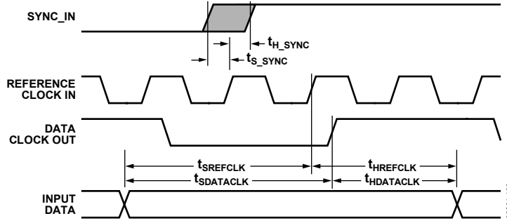
Figure 94. Timing Specifications, PLL Enabled or Disabled, Interpolation = 4x
