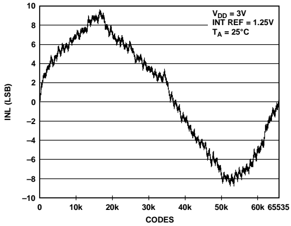
Figure 19. INL AD5668-1
