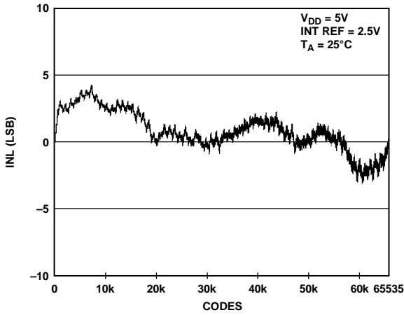
Figure 13. INL AD5668-2/AD5668-3
