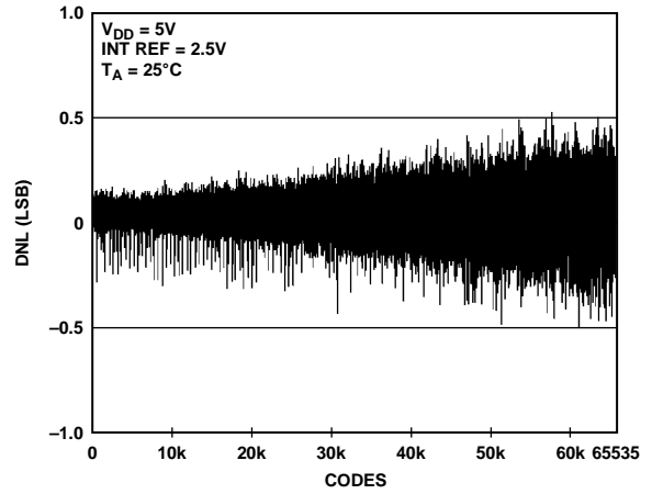
Figure 16. DNL AD5668-2/AD5668-3
