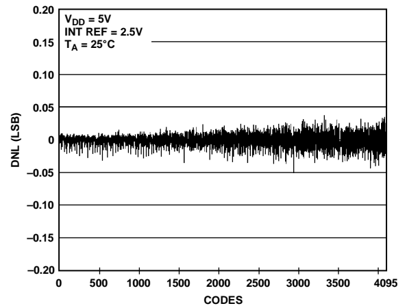
Figure 18. DNL AD5628-2
