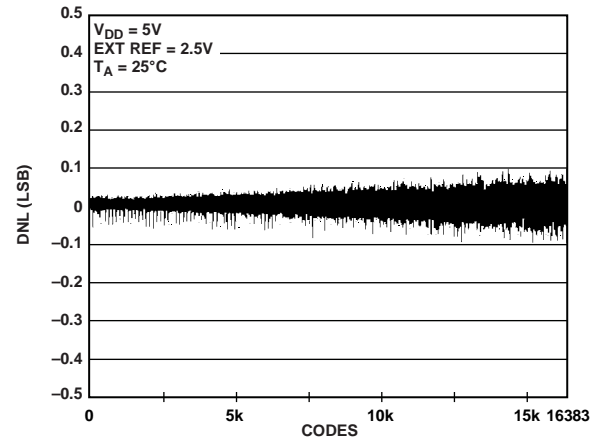
Figure 17. DNL AD5648-2
