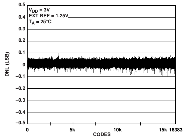
Figure 23. DNL AD5648-1
