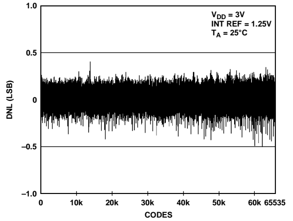
Figure 22. DNL AD5668-1
