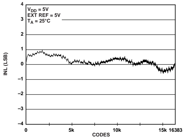
Figure 14. INL AD5648-2
