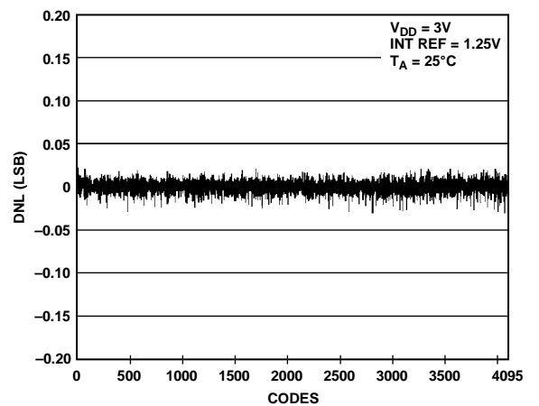
Figure 24. DNL AD5628-1
