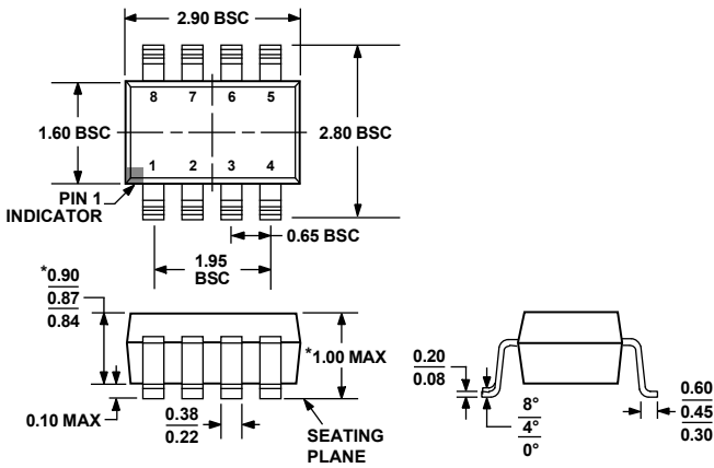
Figure 68. 8-Lead Thin Small Outline Transistor Package [TSOT] (UJ-8) Dimensions shown in millimeters
