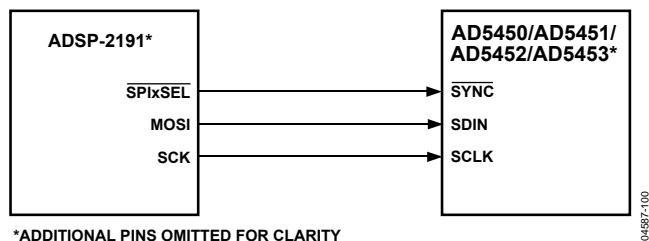
*ADDITIONAL PINS OMITTED FOR CLARITY Figure 56. ADSP-2191 SPI-to-AD5450/AD5451/AD5452/AD5453 Interface
