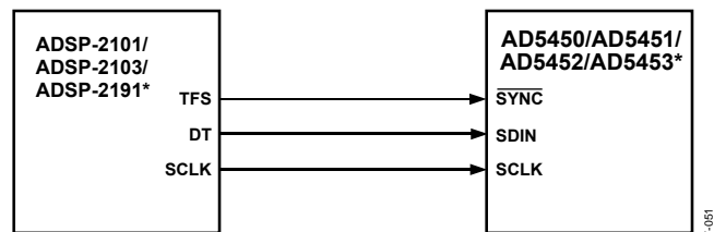
*ADDITIONAL PINS OMITTED FOR CLARITY Figure 57. ADSP-2101/ADSP-2103/ADSP-2191 SPORT-to-AD5450/AD5451/AD5452/AD5453 Interface
