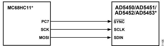
Figure 61. MC68HC11-to-AD5450/AD5451/AD5452/AD5453 Interface
