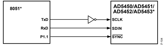
Figure 60. 80C51/80L51-to-AD5450/AD5451/AD5452/AD5453 Interface
