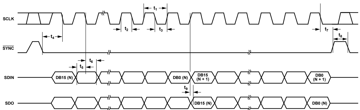
Figure 3. Daisy-Chain Timing Diagram
