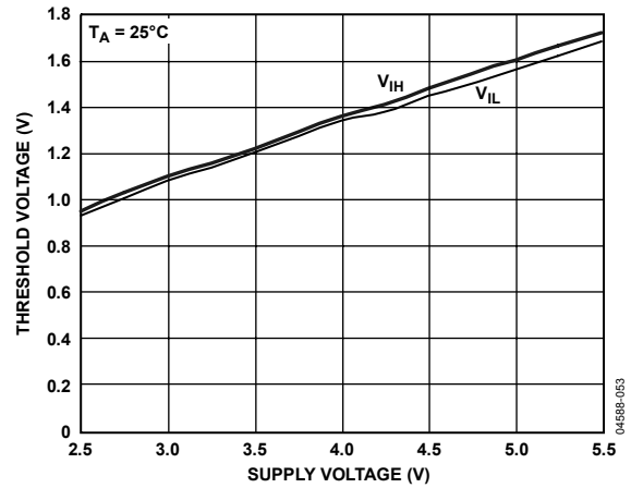
Figure 21. Threshold Voltage vs. Supply Voltage
