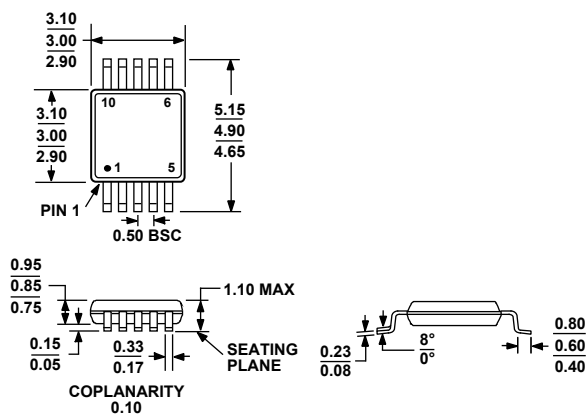
Figure 65. 10-Lead Mini Small Outline Package [MSOP] (RM-10) Dimensions shown in millimeters
