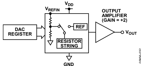
Figure 50. DAC Architecture
