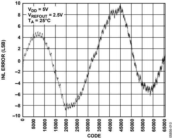
Figure 10. AD5664R-5 INL, Internal Reference
