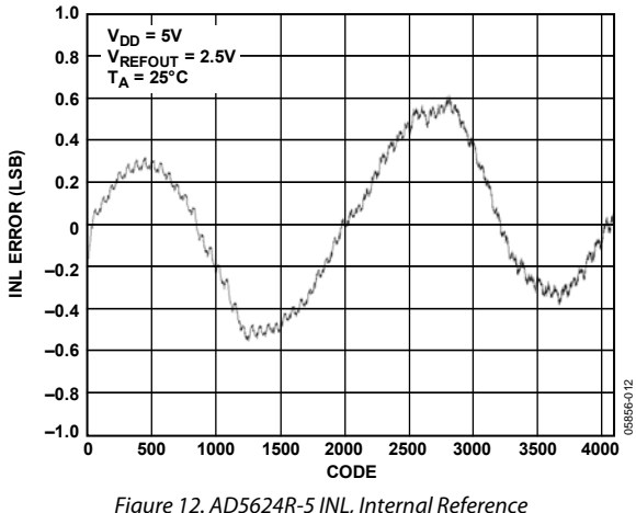
Figure 12. AD5624R-5 INL, Internal Reference
