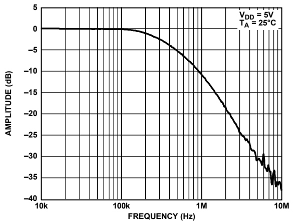
Figure 49. Multiplying Bandwidth
