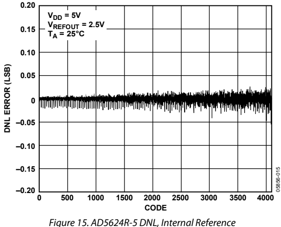
Figure 15. AD5624R-5 DNL, Internal Reference
