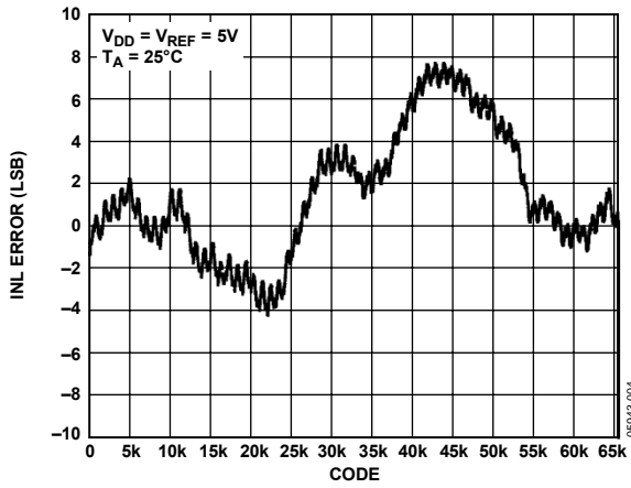
Figure 4. INL AD5664
