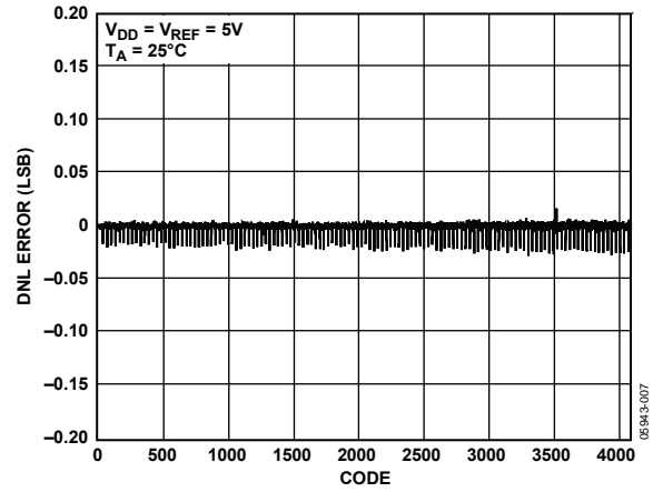
Figure 7. DNL AD5664
