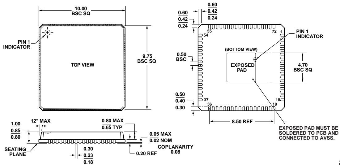
COMPLIANT TO JEDEC STANDARDS MO-220-VNND-4 Figure 44. 72-Lead Lead Frame Chip Scale Package [LFCSP_VQ] 10 mm x 10 mm, Very Thin Quad (CP-72-1) Dimensions shown in millimeters
