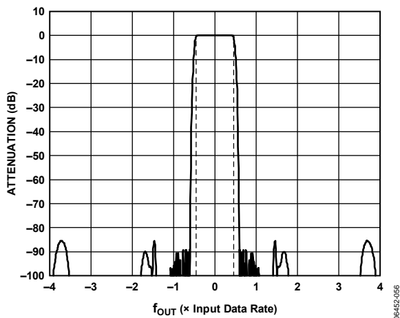
Figure 59. 8× Interpolation, Low-Pass Response to ±4× Input Data Rate (Dotted Lines Indicate 1 dB Roll-Off)
