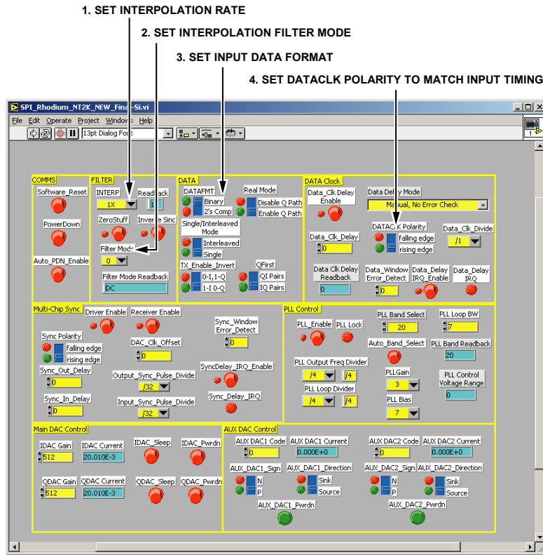
Figure 102. 3-Wire Interface Port Software Window
