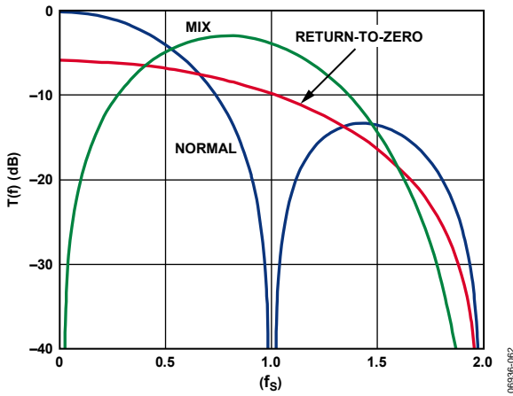
Figure 65. Transfer Function for Each Analog Operating Mode
