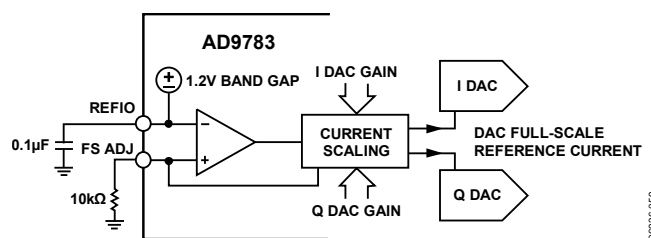
Figure 62. Reference Circuitry
