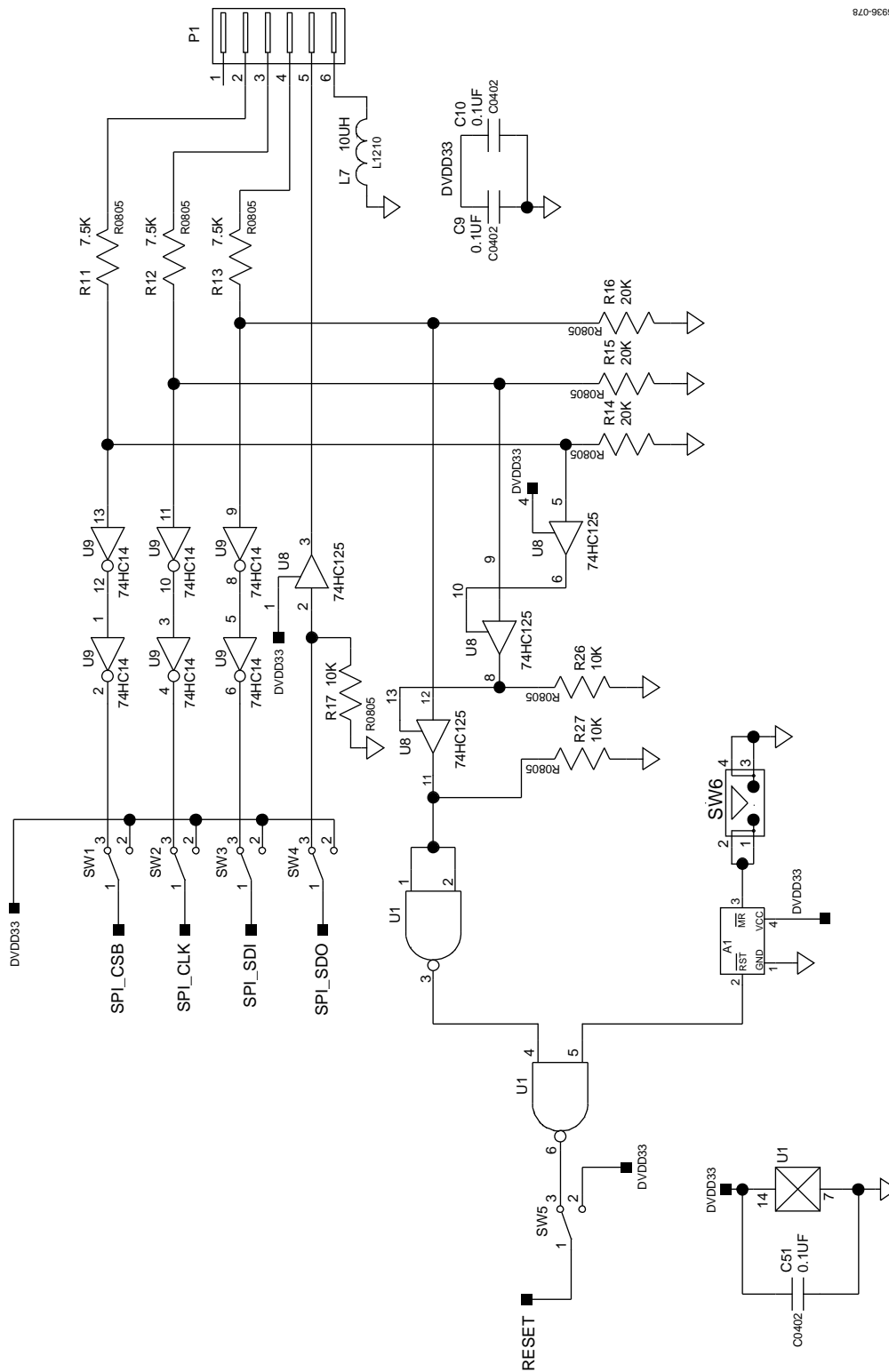
Figure 75. SPI Interface
