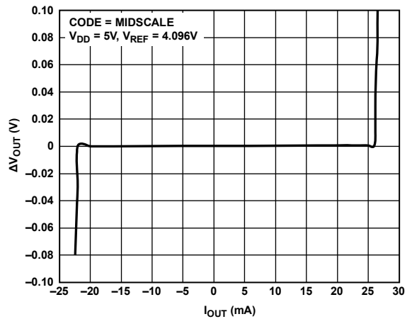
Figure 34. Typical Current Limiting Plot
