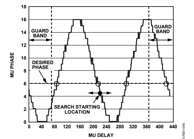
Figure 49. Typical Mu Phase Characteristic Plot at 2.4 GSPS
