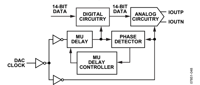
Figure 48. Mu Delay Controller Block Diagram
