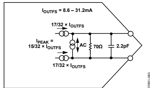
Figure 63. Equivalent DAC Output Circuit
