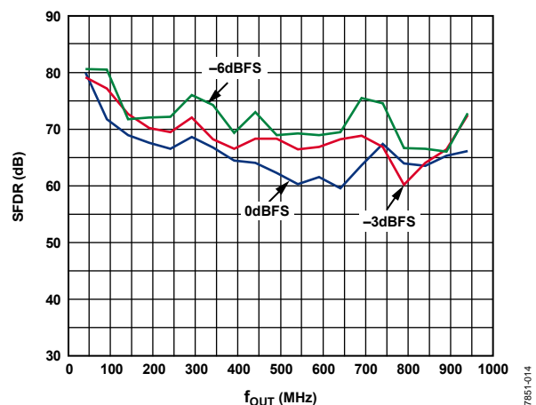
Figure 14. SFDR for Second Harmonic over f_{OUT} vs. Digital Full Scale
