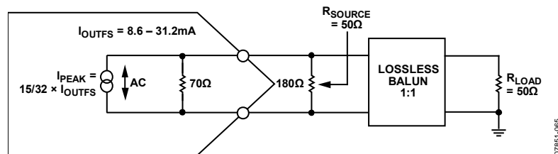
Figure 65. Equivalent Circuit for Determining Maximum Peak Power to a 50\ \Omega Load
