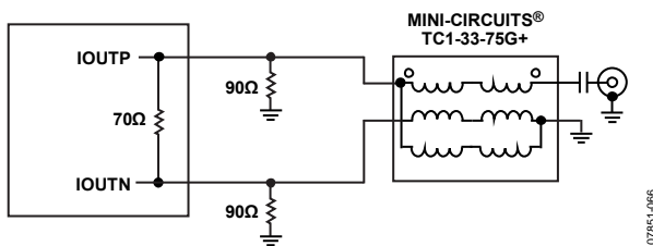
Figure 66. Recommended Balun for Wideband Applications with Upper Bandwidths of up to 2.2 GHz
