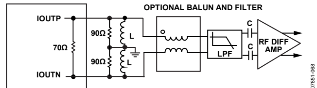
Figure 68. Interfacing the DAC Output to the Self-Biased Differential Gain Stage
