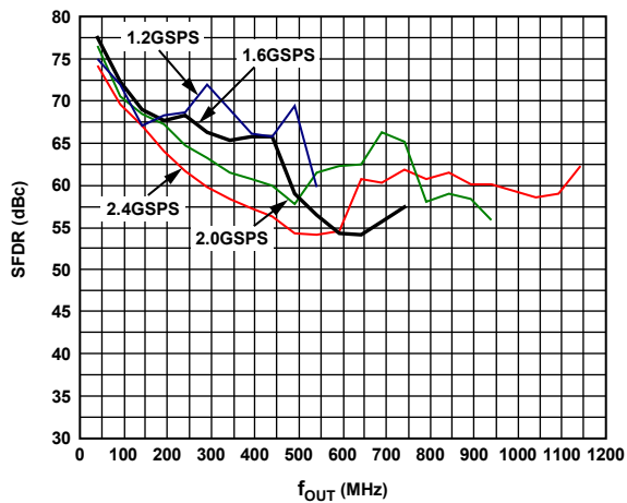
Figure 8. SFDR vs. f_{OUT} over f_{DAC}
