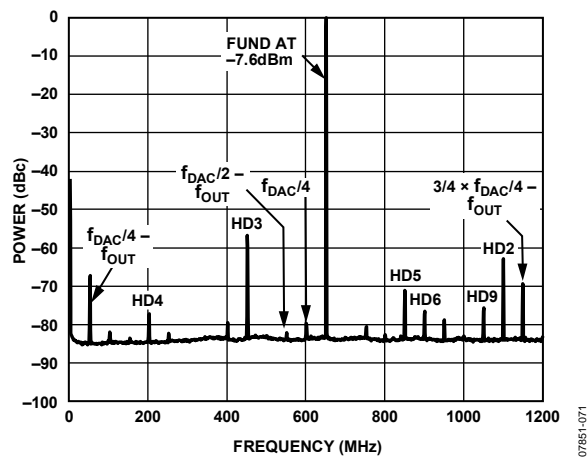
Figure 71. Spectral Plot
