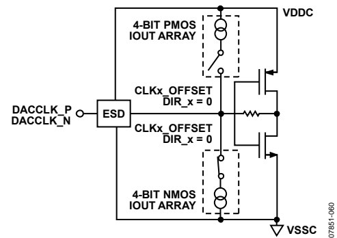
Figure 58. Clock Input and Common-Mode Control
