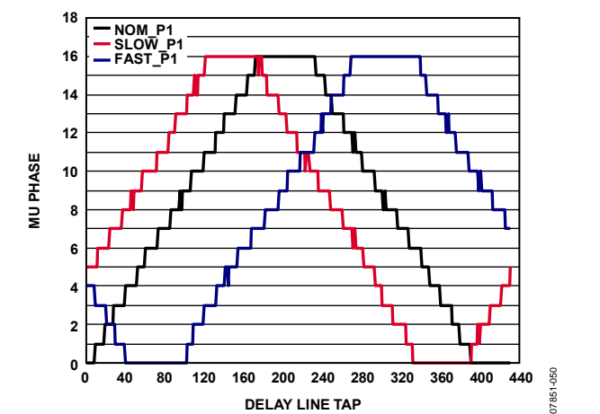
Figure 50. Mu Phase Characteristics of Three Devices from Different Process Lots at 1.2 GSPS
