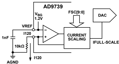
Figure 62. Voltage Reference Circuit
