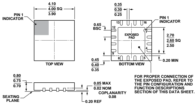
Figure 55. 16-Lead Lead Frame Chip Scale Package [LFCSP_WQ] 4 mm × 4 mm Body, Very Very Thin Quad (CP-16-17)
