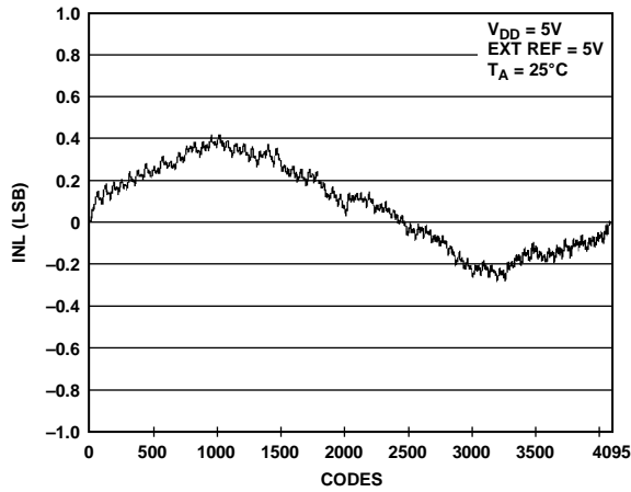
Figure 6. INL AD5629R—External Reference
