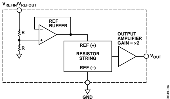
Figure 48. DAC Architecture for External Reference Configuration
