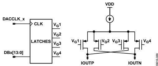
Figure 169. AD9739A Quad-Switch Architecture
