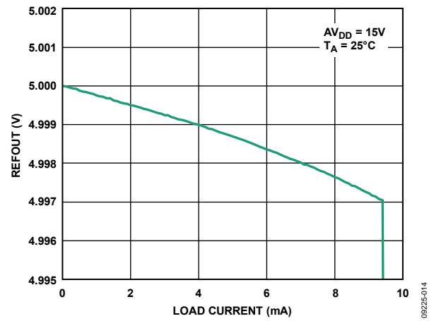
Figure 42. REFOUT vs. Load Current
