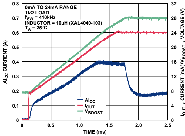
Figure 59. A_{I_{CC}} Current vs. Time for 24 mA Step Through 1 kΩ Load with External 51 kΩ Compensation Resistor
