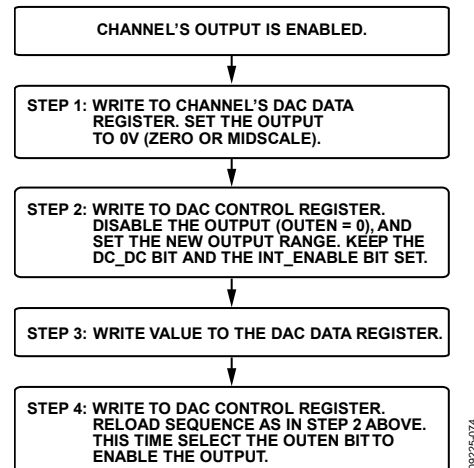
Figure 52. Steps for Changing the Output Range
