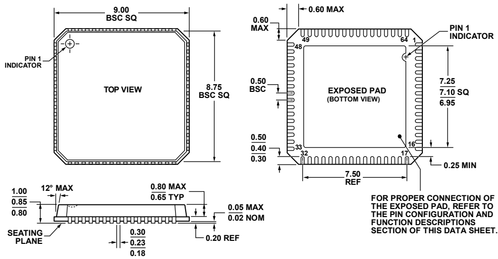
Figure 66. 64-Lead Lead Frame Chip Scale Package [LFCSP_VQ] 9 mm × 9 mm Body, Very Thin Quad (CP-64-3)
