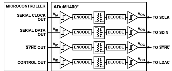
Figure 65. Isolated Interface
