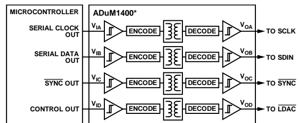
Figure 88. Isolated Interface
