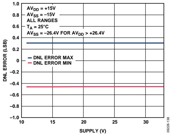
Figure 21. Differential Nonlinearity Error vs. AV_{DD}/|AV_{SS}|
