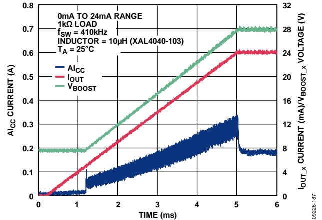
Figure 85. I_{CC} Current vs. Time for 24 mA Step Through 1 k \Omega Load with Slew Rate Control
