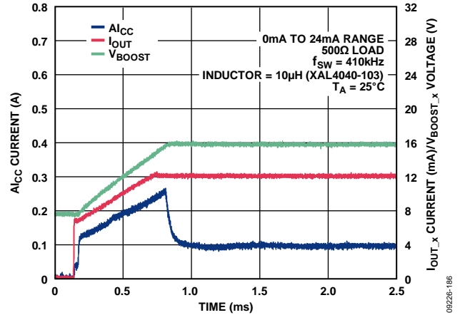
Figure 84. I_{CC} Current vs. Time for 24 mA Step Through 500 \Omega Load with External 51 k \Omega Compensation Resistor
