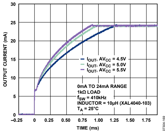
Figure 50. Output Current Settling with DC-to-DC Converter vs. Time and AVcc (See Figure 78)
