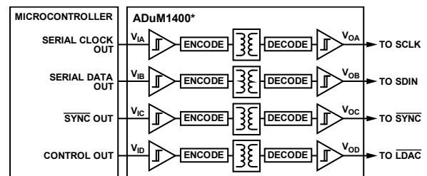
Figure 86. Isolated Interface
