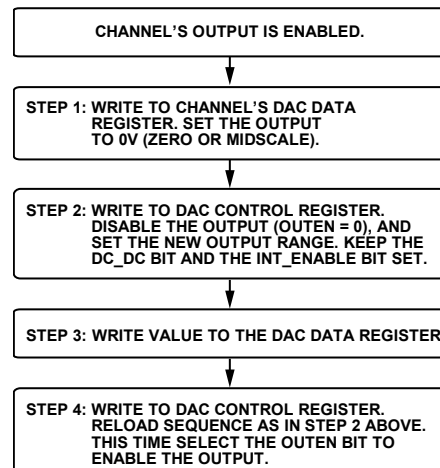
Figure 75. Steps for Changing the Output Range
