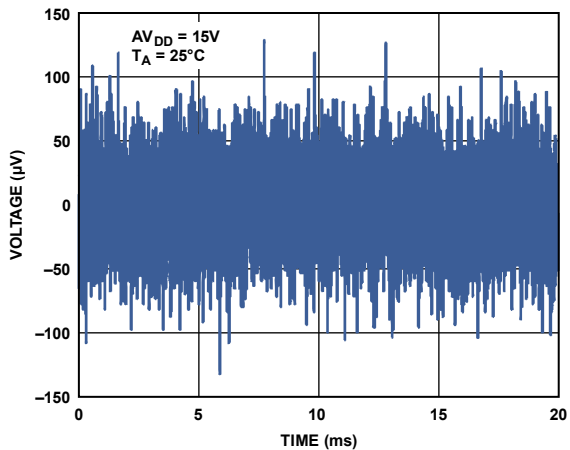
Figure 39. REFOUT Output Noise (100 kHz Bandwidth)
