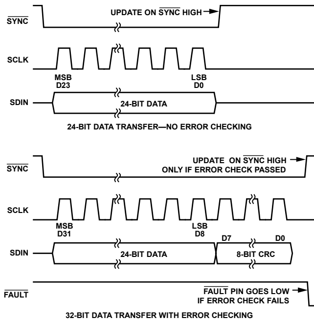
Figure 53. PEC Timing
