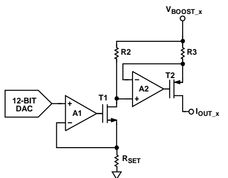
Figure 48. Voltage-to-Current Conversion Circuitry
