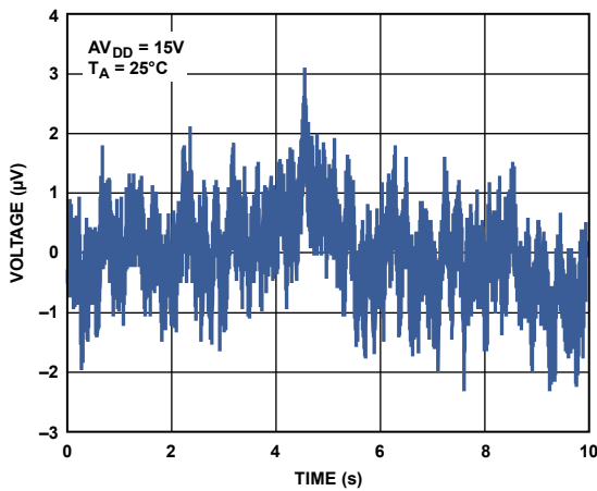
Figure 38. REFOUT Output Noise (0.1 Hz to 10 Hz Bandwidth)
