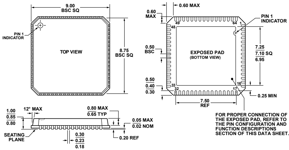
Figure 65. 64-Lead Lead Frame Chip Scale Package [LFCSP_VQ] 9 mm × 9 mm Body, Very Thin Quad (CP-64-3) Dimensions shown in millimeters
