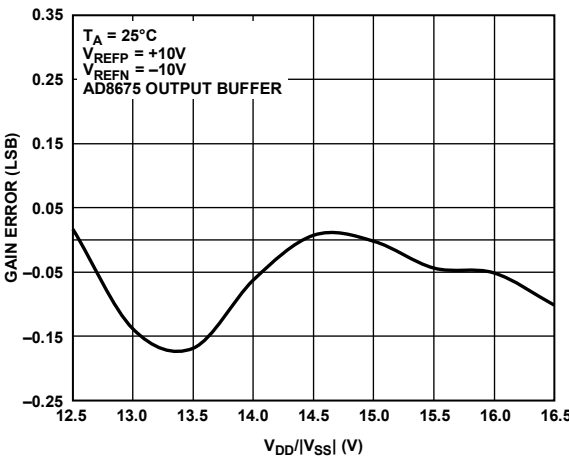
Figure 26. Gain Error vs. Supply Voltage, ±10 V Span
