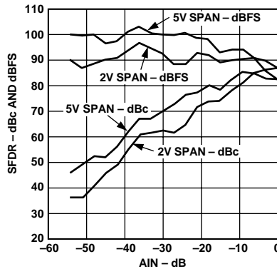
Figure 9. Single Tone SFDR ( f_{IN} = 5.0 \text{ MHz} , V_{CM} = 2.5 \text{ V} )
