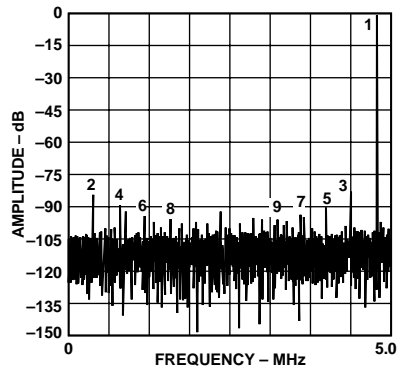
Figure 7. Typical FFT, f_{IN} = 5.0 \text{ MHz} (Input Span = 2 V, V_{CM} = 2.5 \text{ V} )
