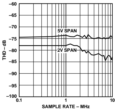
Figure 8. THD vs. Sample Rate ( f_{IN} = 5.0 \text{ MHz} , A_{IN} = -0.5 \text{ dBFS} , V_{CM} = 2.5 \text{ V} )
