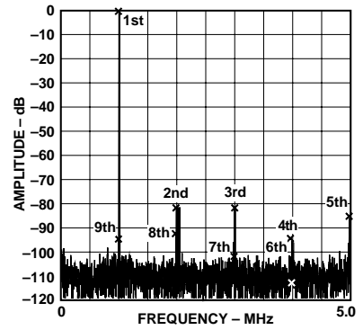
Figure 4. Typical FFT, f_{IN} = 1.0 \text{ MHz} (Input Span = 5 V, V_{CM} = 2.5 \text{ V} )
