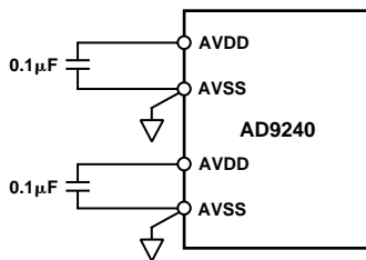
Figure 49. Analog Supply Decoupling
