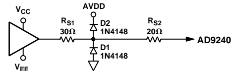
Figure 31. Simple Clamping Circuit
