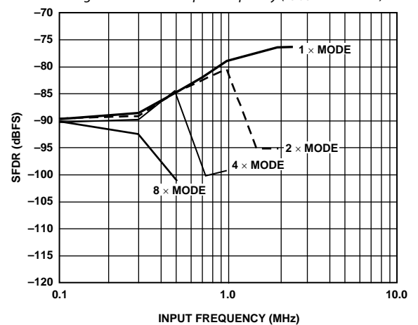
Figure 22. SFDR vs. Input Frequency ( f_{\text{CLOCK}} = 10 MSPS)
