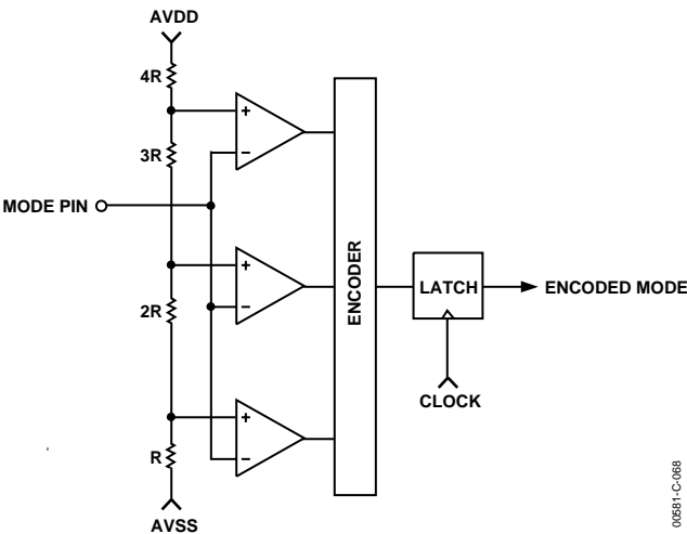
Figure 68. Simplified Mode Pin Circuitry
