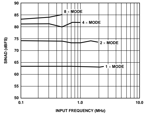
Figure 20. SINAD vs. Input Frequency ( f_{\text{CLOCK}} = 10 MSPS)
