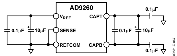
Figure 67. Recommended Reference Decoupling Network
