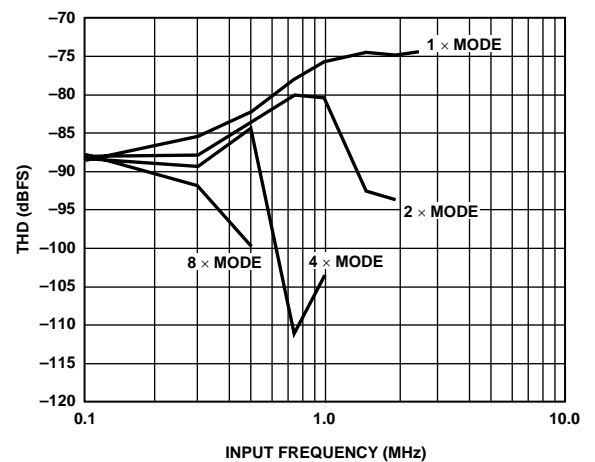
Figure 21. THD vs. Input Frequency ( f_{\text{CLOCK}} = 10 MSPS)
