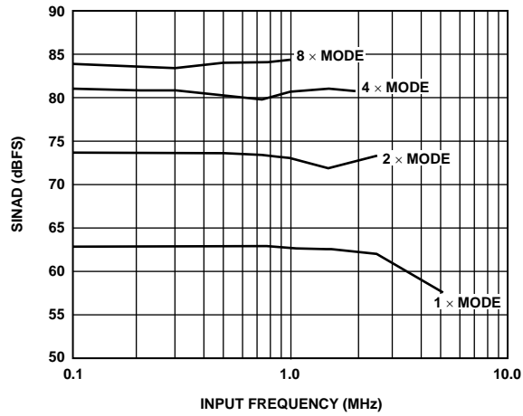
Figure 17. SINAD vs. Input Frequency ( f_{\text{CLOCK}} = 20 MSPS) 8x SINAD performance limited by noise contribution of input differential op amp driver
