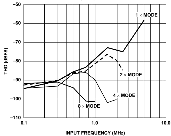
Figure 18. THD vs. Input Frequency ( f_{\text{CLOCK}} = 20 MSPS)
