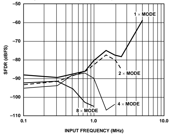
Figure 19. SFDR vs. Input Frequency ( f_{\text{CLOCK}} = 20 MSPS)
