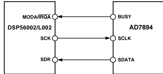
Figure 9. AD7894 to DSP56002/L002 Interface
