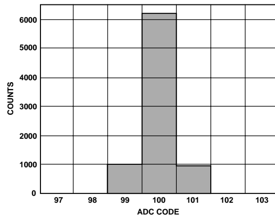
Figure 10. Histogram of 8192 Conversions of a DC Input
