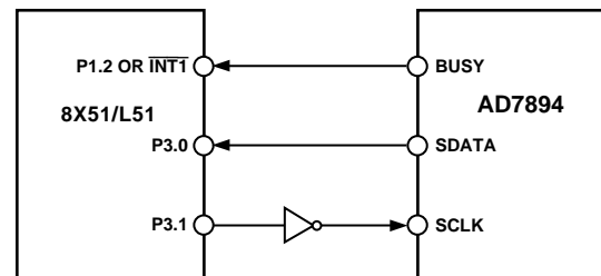
Figure 6. AD7894 to 8X51/L51 Interface
