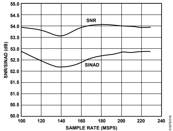
Figure 16. SNR/SINAD vs. Sample Rate; A_{IN} = 70 MHz
