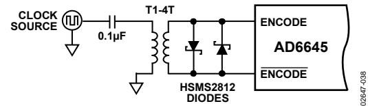
Figure 38. Crystal Clock Oscillator, Differential Encode
