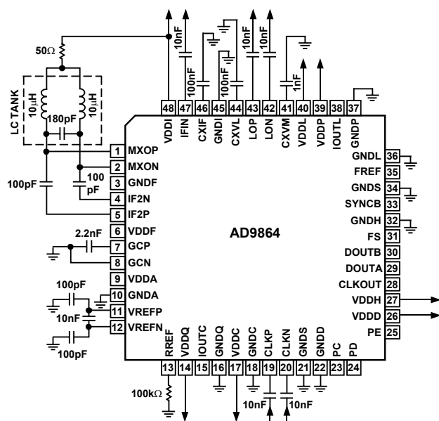
Figure 70. Example Circuit Showing Recommended Component Values
