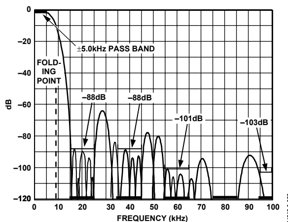
Figure 52. Decimation Filter Frequency Response for f_{OUT} = 20 kSPS ( f_{CLK} = 18 MHz, OSR = 900 )
