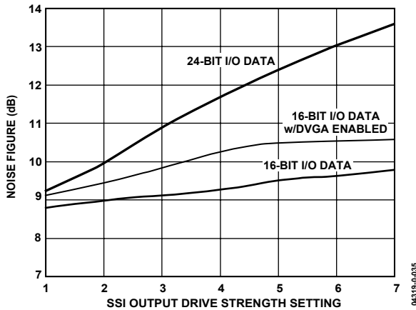
Figure 35. NF vs. SSI Output Drive Strength ( V_{DDX} = 3.0V , F_{CLK} = 18\text{ MSPS} , BW = 75\text{ kHz} )
