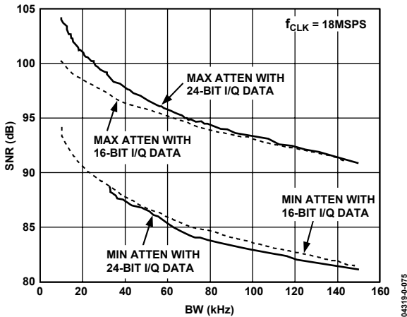
Figure 74. Hung Mixer SNR vs. BW and VGA
