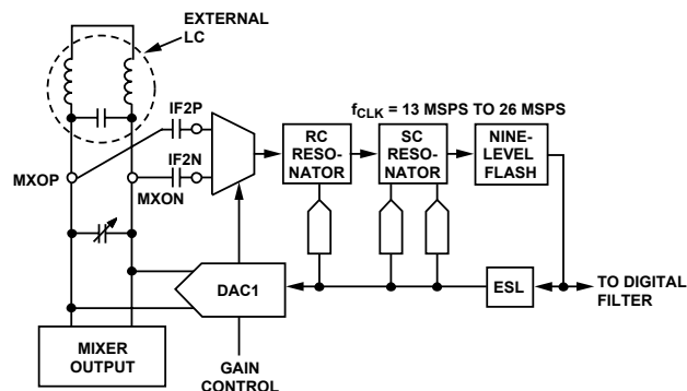
Figure 46. Equivalent Circuit of Sixth Order Band-Pass \Sigma - \Delta Modulator
