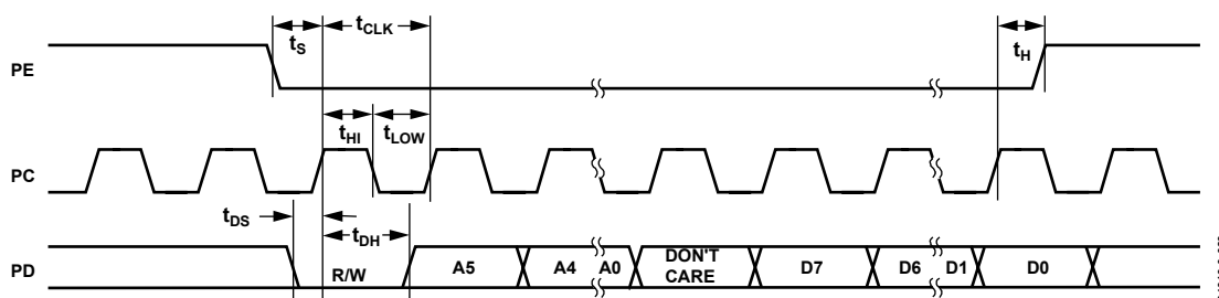
Figure 29. SPI Write Operation Timing
