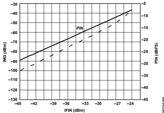
Figure 20. IMD vs. IFIN ( f_{CLK} = 18 MSPS)
