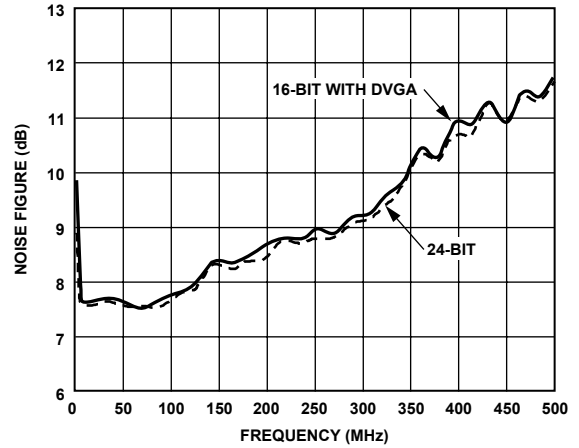
Figure 24. Noise Figure vs. Frequency (Minimum Attenuation, f_{CLK} = 18 MSPS, BW = 10 kHz)
