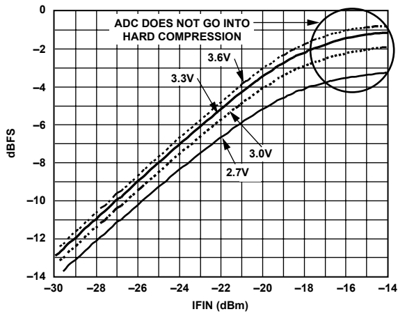
Figure 10. Gain Compression vs. IFIN
