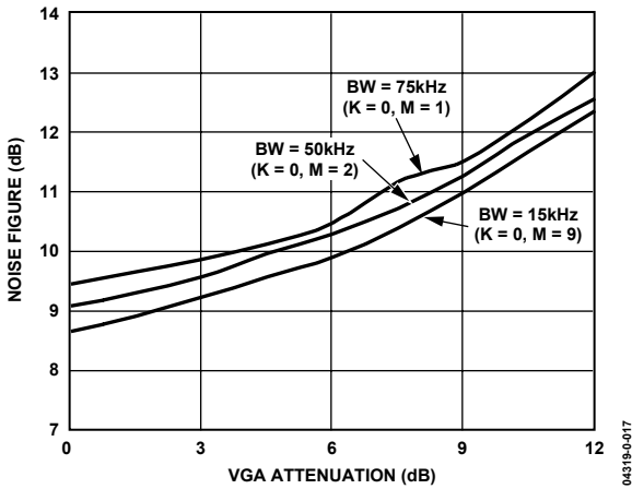
Figure 16. Noise Figure vs. VGA Attenuation ( f_{CLK} = 18 MSPS)
