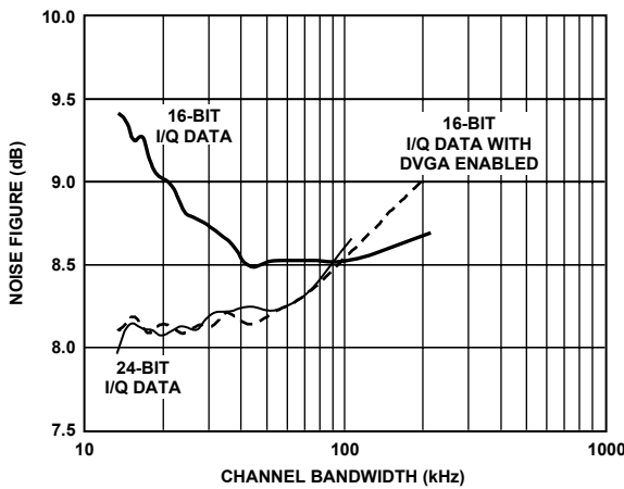
Figure 11. Noise Figure vs. BW (Minimum Attenuation, f_{CLK} = 13\text{ MSPS} )
