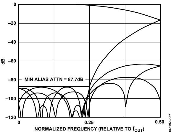
Figure 56. Folded Decimator Frequency Response for K = 0
