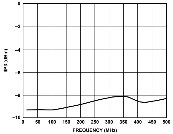
Figure 25. Input IIP3 vs. Frequency ( f_{CLK} = 18 MSPS)
