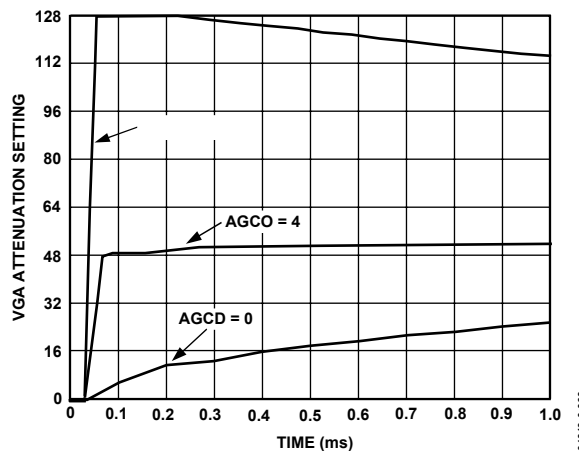
Figure 62. AGC Response for Different AGCO Settings with f_{CLK} = 18 MSPS, f_{CLKOUT} = 300 KSPS, Decimate by 60 and AGCA = AGCD = 0
