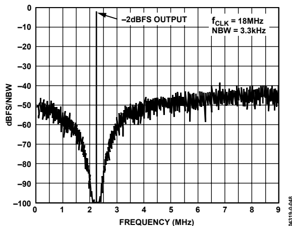
Figure 47. Measured Undecimated Spectral Output of \Sigma - \Delta Modulator ADC with f_{CLK} = 18 MSPS and Noise Bandwidth of 3.3 kHz
