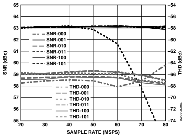
Figure 84. SNR and THD Performance vs. f_{DC} and ADC Bias Setting with RxPGA = 0 dB, f_{IN} = 10 MHz, A_{IN} = -1 dBFS
