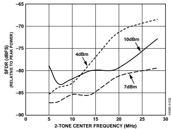
Figure 32. 2-Tone Worst Spur Frequency Sweep vs. Peak Power with f_{DATA} = 80 MSPS, 2× Interpolation
