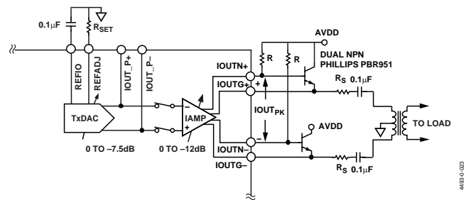
Figure 65. Voltage-Mode Operation
