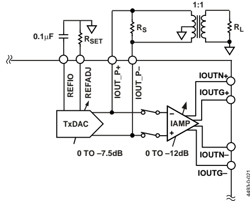
Figure 63. TxDAC Output Directly via Center-Tap Transformer
