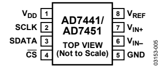
Figure 6. 8-Lead SOT-23 Pin Configuration
