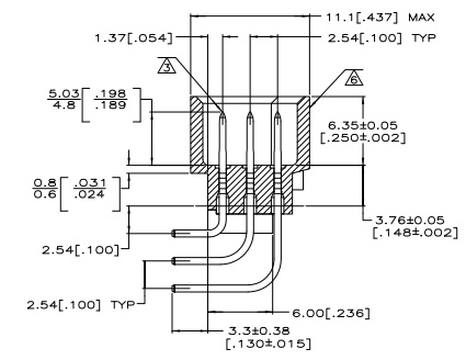
SECTION X-X
