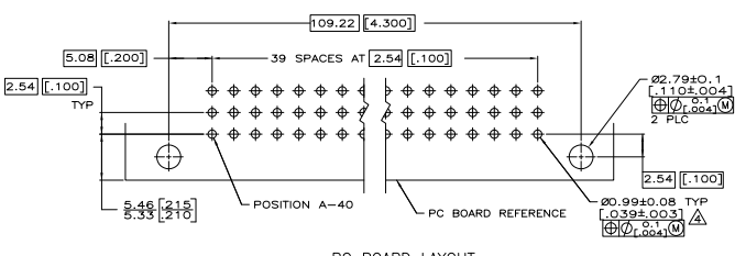
PC BOARD LAYOUT
