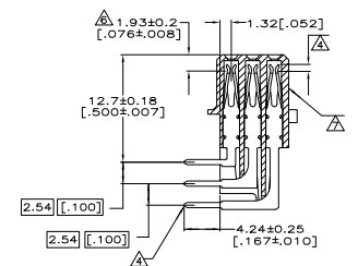
SECTION Y-Y
