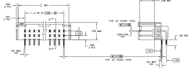
SECTION X-X
