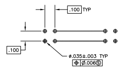
RECOMMENDED HOLE LAYOUT
