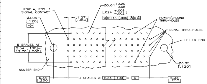
RECOMMENDED CURCUIT PATTERN PER ANSI/IPC-D-300 TYPE II, CLASS C (COMPONENT SIDE)
