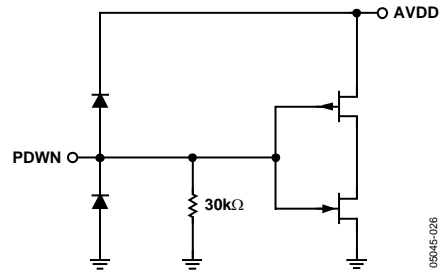
Figure 26. Power-Down Input
