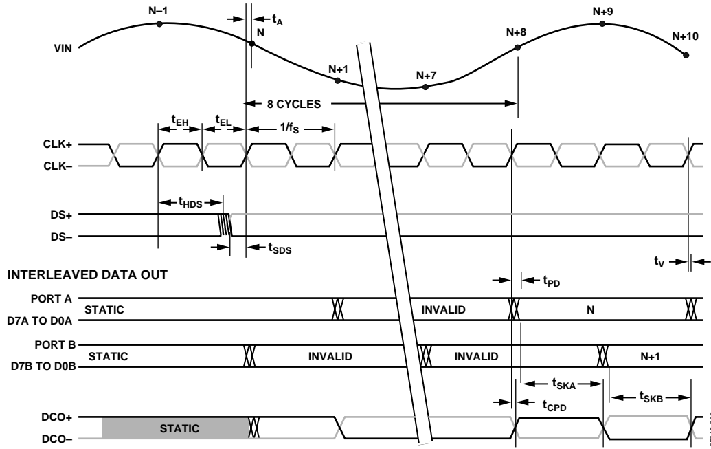
Figure 2. Timing Diagram
