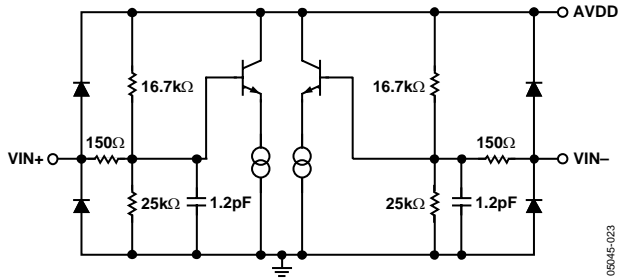
Figure 23. Analog Inputs
