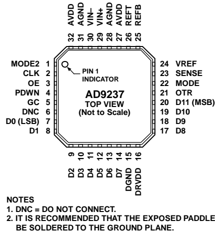
Figure 3. Pin Configuration
