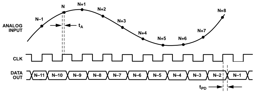
Figure 2. Timing Diagram
