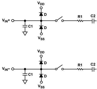
NOTES 1. V_{IN+} CAN BE V_{IN0} OR V_{IN2} , AND V_{IN-} CAN BE V_{IN1} OR V_{IN3} . Figure 30. Equivalent Analog Input Circuit (Differential)
