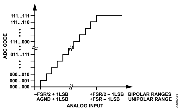
Figure 28. Straight Binary Transfer Characteristic
