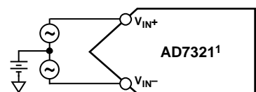
Figure 34. True Differential Inputs
