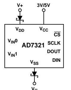
Figure 53. Schottky Diode Connection
