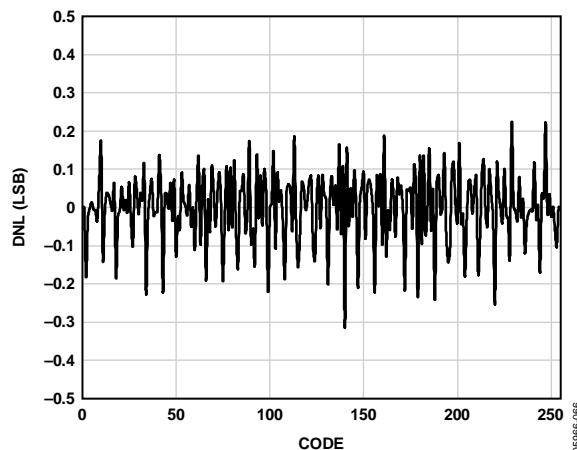
Figure 30. DNL, f_{\text{IN}} = 2.4 \text{ MHz} , f_{\text{SAMPLE}} = 100 \text{ MSPS}
