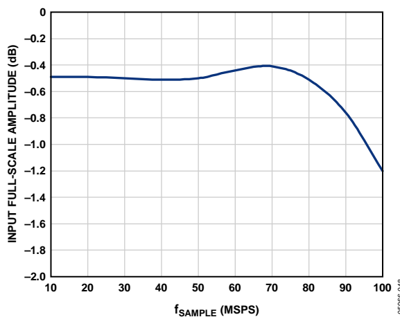
Figure 32. Input Full-Scale Amplitude vs. f_{\text{SAMPLE}}
