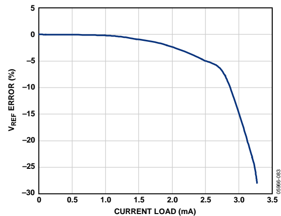
Figure 55. V_{REF} Error vs. Load
