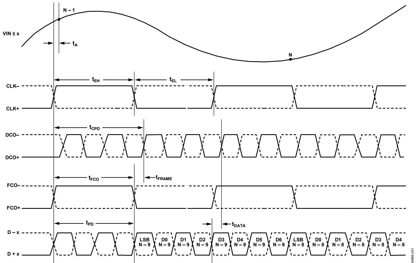
Figure 4. 8-Bit Data Serial Stream, LSB First
