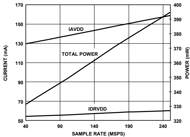
Figure 31. AD9230-210 Power Supply Current vs. Sample Rate
