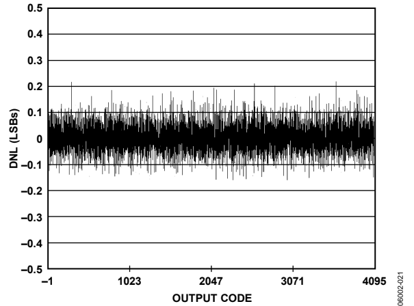
Figure 21. AD9230-170 DNL; 170 MSPS
