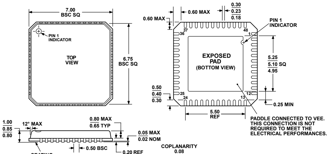
Figure 49. 48-Lead Lead Frame Chip Scale Package [LFCSP_VQ] 7 mm x 7 mm Body, Very Thin Quad (CP-48-1)
