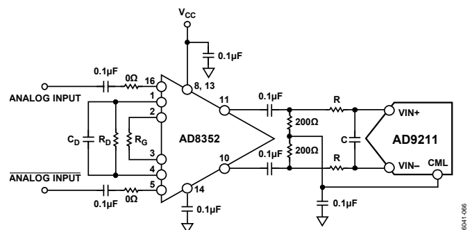
Figure 41. Differential Input Configuration Using the AD8352
