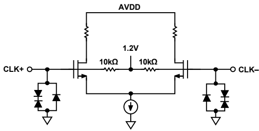
Figure 33. Clock Inputs
