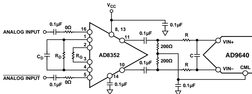
Figure 50. Differential Input Configuration Using the AD8352
