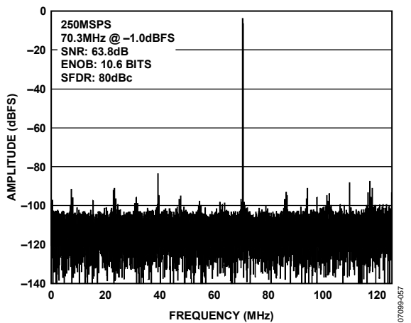
Figure 31. AD9626-250 64k Point Single-Tone FFT; 250 MSPS, 70.3 MHz
