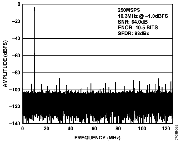
Figure 30. AD9626-250 64k Point Single-Tone FFT; 250 MSPS, 10.3 MHz
