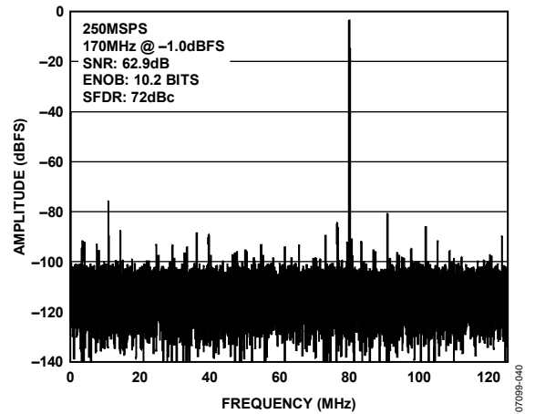
Figure 32. AD9626-250 64k Point Single-Tone FFT; 250 MSPS, 170.3 MHz
