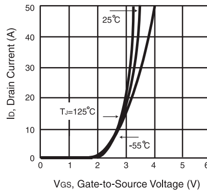
Figure 2. Transfer Characteristics
