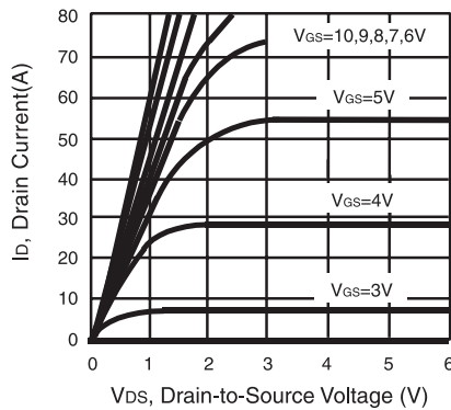
Figure 1. Output Characteristics
